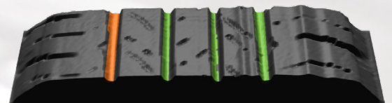
TreadReader™ 3D tyre scan
